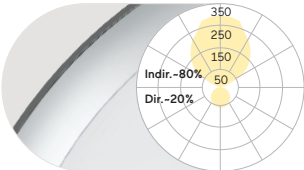
Opal Diffuser | Direct-Indirect
