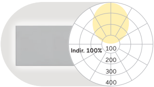
Indirect Optic | Indirect
