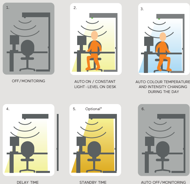
FUNCTIONAL DIAGRAM
