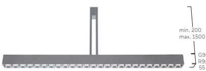
Twin Rod Suspension
