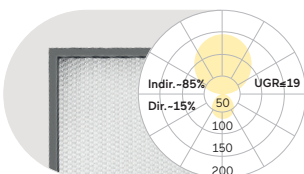
Microprismatic | Direct-Indirect | Sharp Edge
