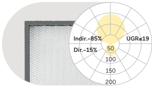
CF2: Microprismatic | Direct-Indirect | Sharp Edge
