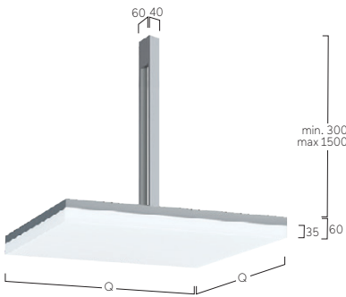
Twin Rod Suspension
