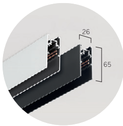
Suspended Track Linear: X-LPQ-840M-L2000-B [BLACK] X-LPQ-840M-L2000-W [WHITE]
